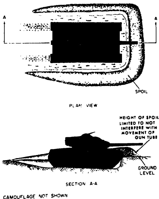
Figure 1-28. Dug-in emplacement for self-propelled weapons.
